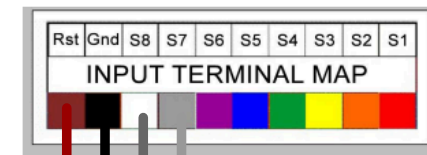
When any S1 to S8 input is shorted to GND, then will trigger the alarm
