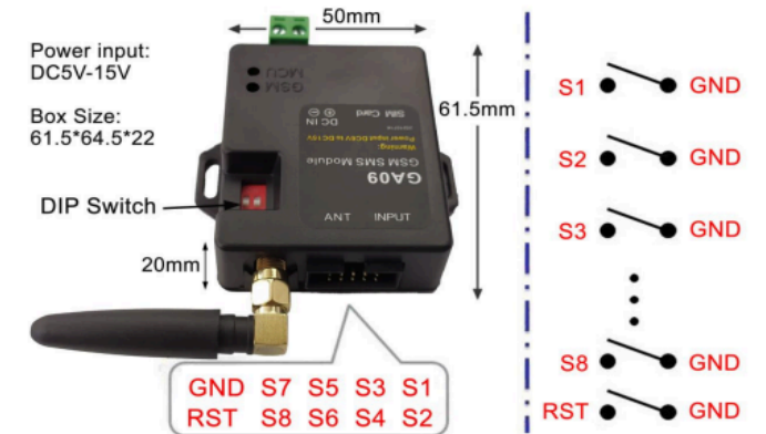
When any S1 to S8 input is shorted to GND, then will trigger the alarm
